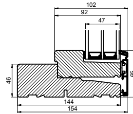
Fastskruet ramme/ Dummy sash
