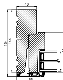
Fastskruet ramme/ Fixed sash
