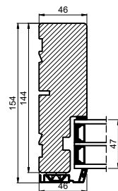
Fast karm/ Fixed frame
