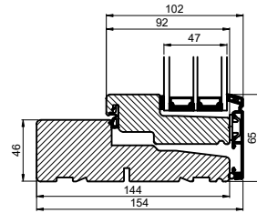
Vindue/ Window
