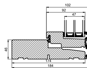
Fastskruet ramme/ Fixed sash
