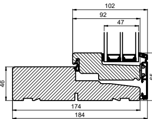
Fast karm/ Fixed frame
