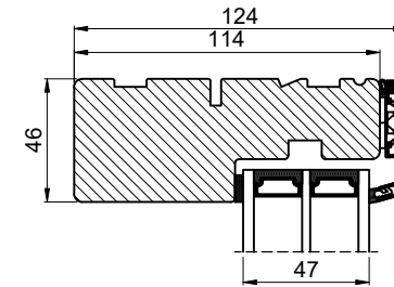
Lodret snit A / Vertical section A
