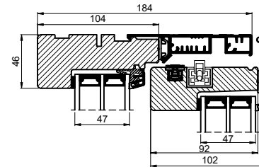
Lodret snit B/ Vertical section B
