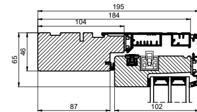
Lodret snit C/ Vertical section C
